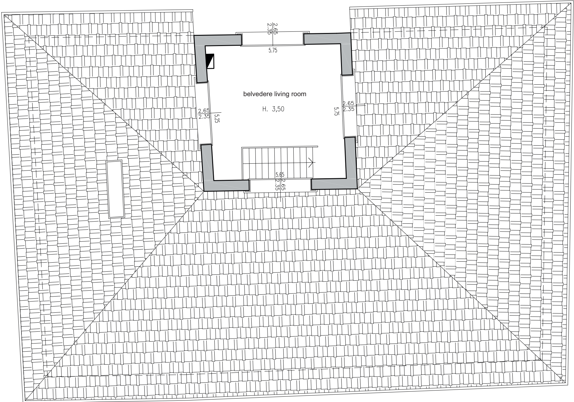
TOWER
