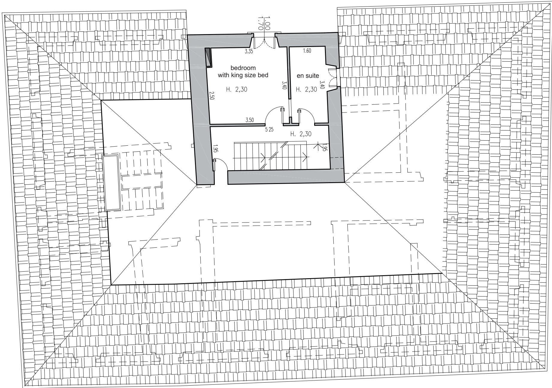
MEZANINE
