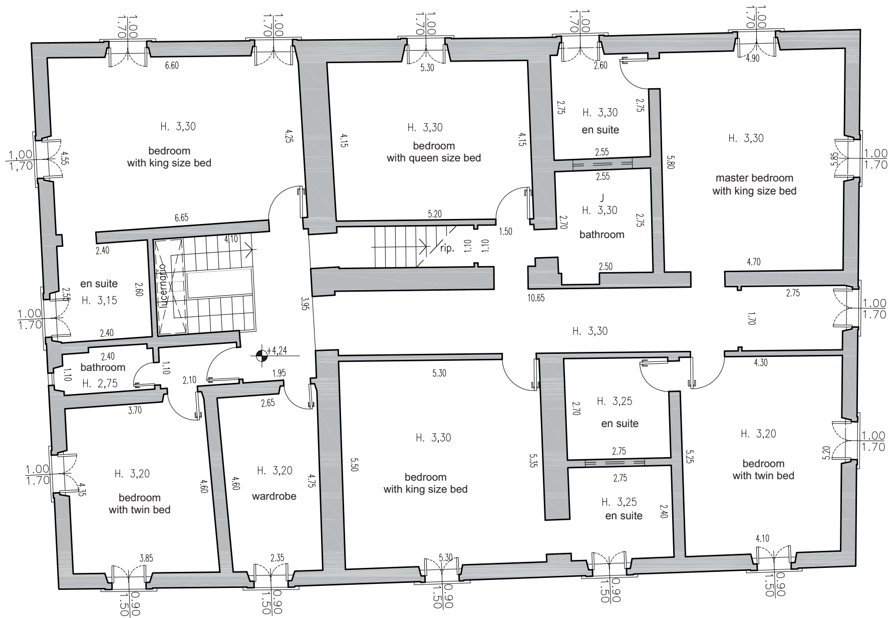
FIRST FLOOR
